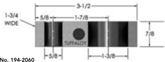
Part No. 194-2060
